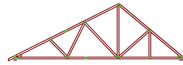
DUAL PITCH
