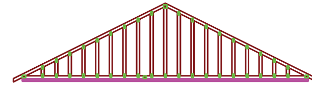
COMMON GABLE END
